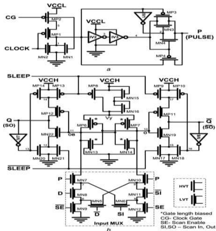
Fig 2.1 Dual-Edge Triggered State Retention Scan Flip-Flop (DET SRSFF).
