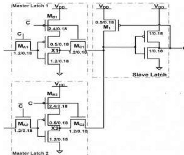
Fig 2.3 Flip-Flop circuitry. Master Latch 1 is referred to as the upper path, and Master Latch 2 is referred to as the lower path in this paper.
