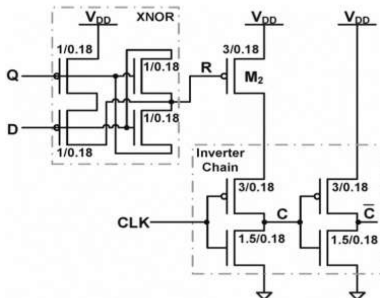
Fig 2.2 Clock-gating and internal clock generating circuitry.
