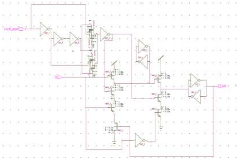
Fig 3.1 Power gated double edge triggered flip flop
