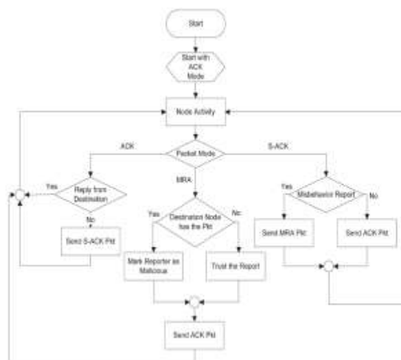
Figure 3: System Flow of EAACK
