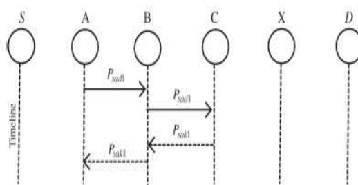
Figure 2: S-Ack Scheme Node C is Required to Send Back an Acknowledge Packet to Node B
