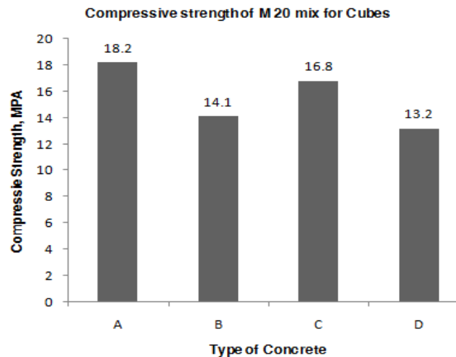
Figure 1 Compressive Strength of 7 Days for Cube
