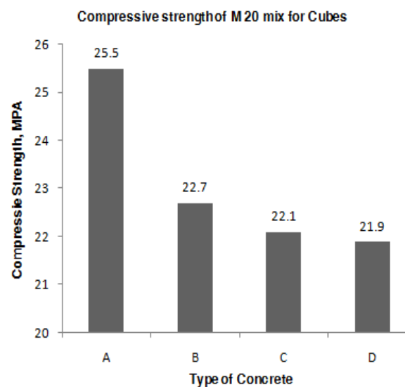
Figure 2 Compressive Strength of 28 Days for Cube
