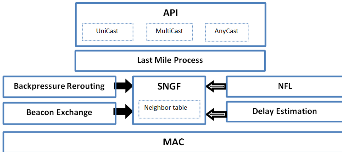
Figure.2 SPEED Protocol
