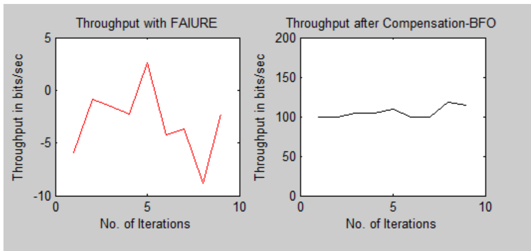
Figure. 4 Throughput
