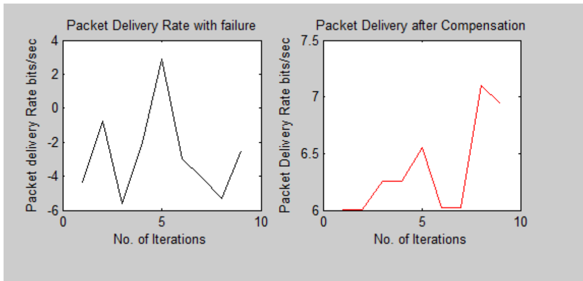
Figure.6 Packet delivery
