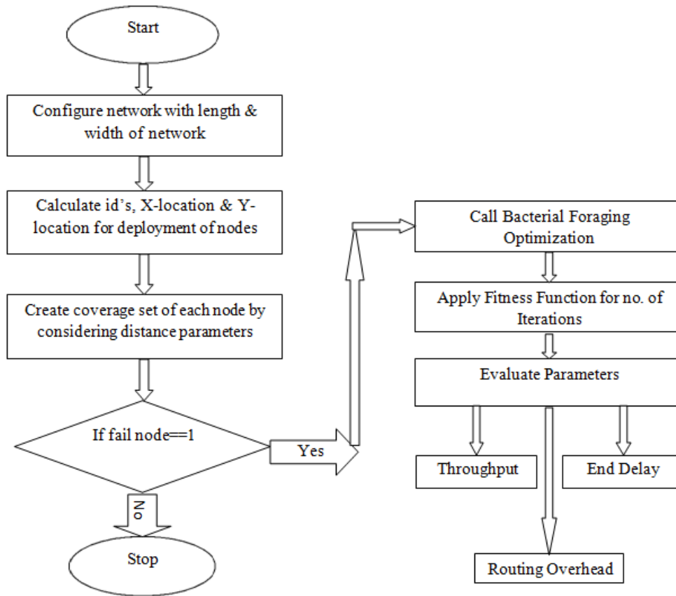
Figure.3 Proposed Model
