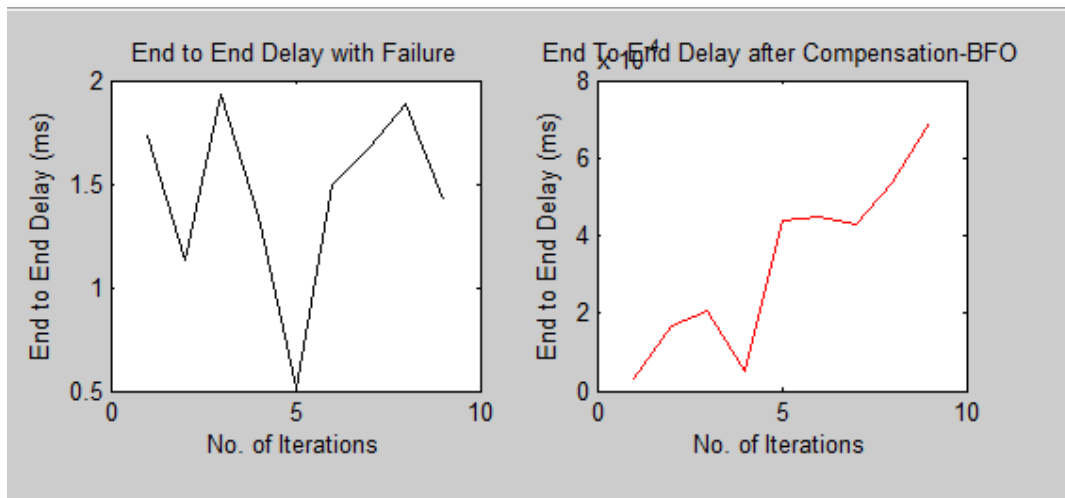
Figure.5 End Delay
