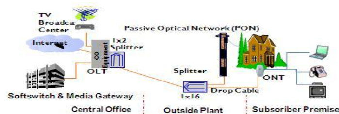
Fig.2 PON Architecture. [22].
