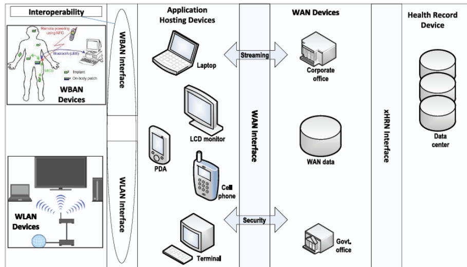
FIGURE 6. Continua Health Alliance's framework-based simplified reference architecture.
