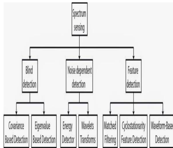
Figure 3: Spectrum Sensing Techniques
