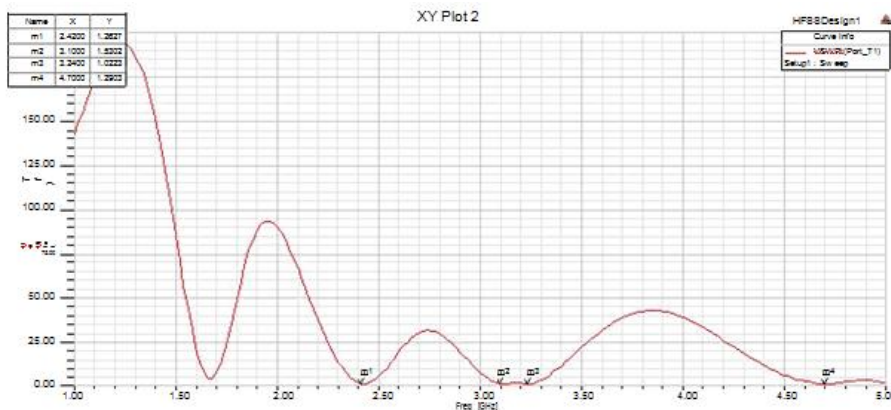
Fig.5 VSWR v/s Frequency Plot of slotted antenna
