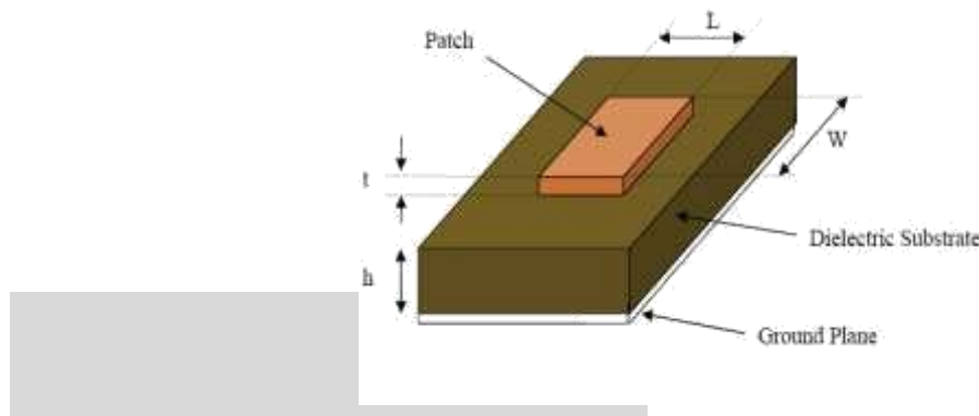
Structure of a Microstrip Patch Antenna
