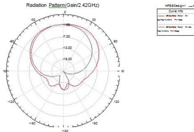
Fig.6 Gain at the 2.42 GHz Frequency
