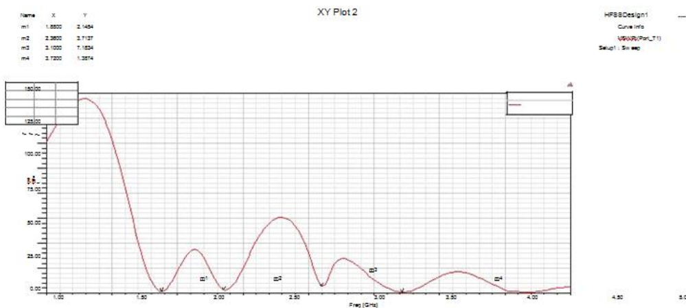
Fig.4 VSWR v/s Frequency Plot of without slot antenna
