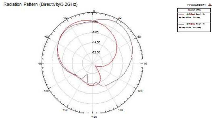
Fig.9 Directivity at the 3.24 GHz Frequency
