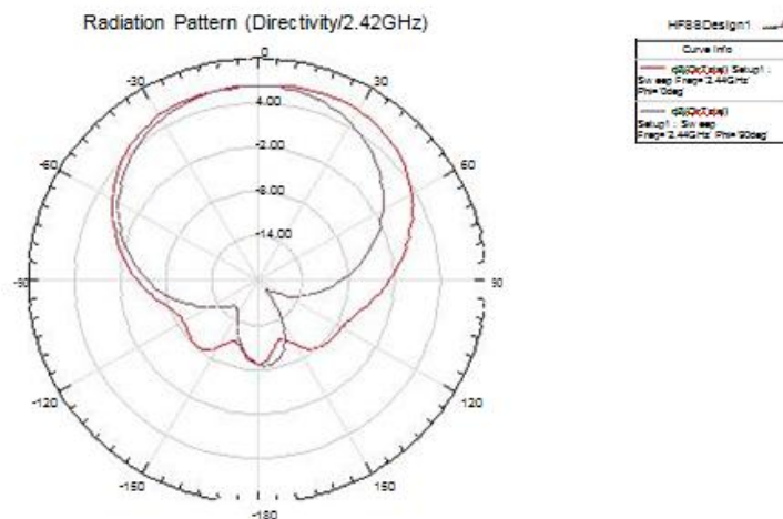
Fig.8 Directivity at the 2.42 GHz Frequency
