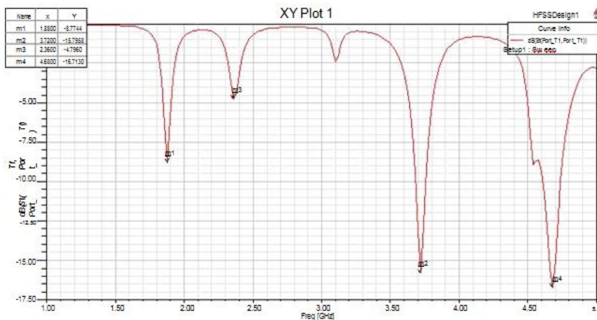
Fig.2 Return Loss of Microstrip Patch Antenna without slot
