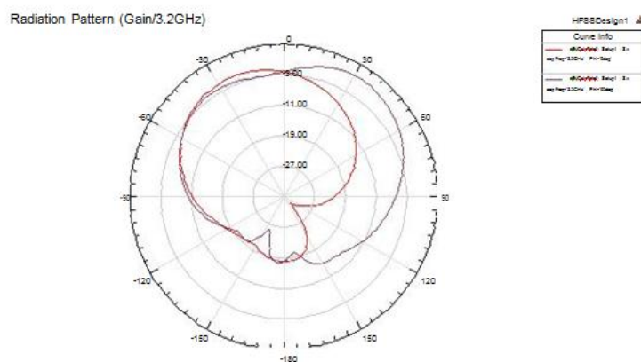
Fig.7 Gain at the 3.24 GHz Frequency
