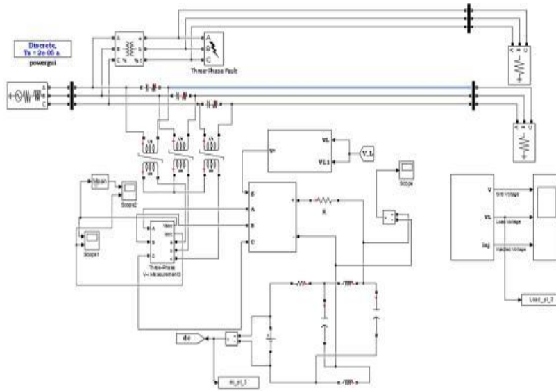
Figure5: Simulation Circuit of System with DVR
