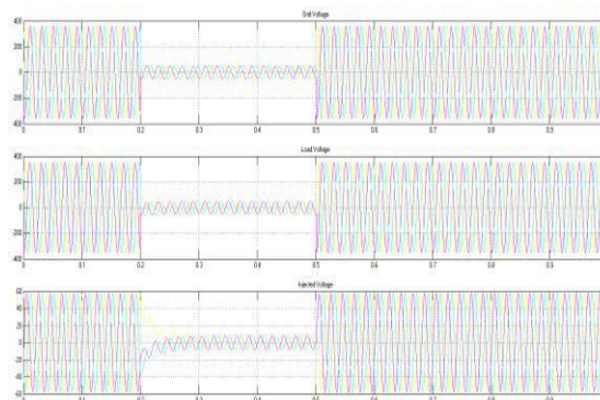
Figure7: a) Source Voltage b) Load Voltage c) Injected Voltage without connecting DVR
