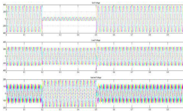
Figure 8: a) Source Voltage b) Load Voltage c) Injected Voltage with DVR
