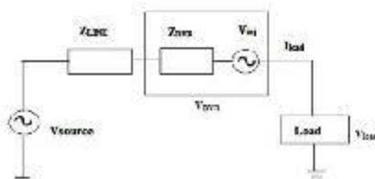
Figure2: Equivalent circuit
