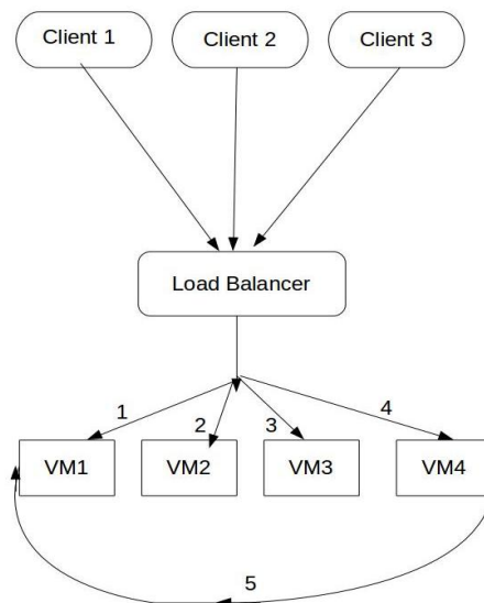
Fig.1 RoundRobin Load Balancer
