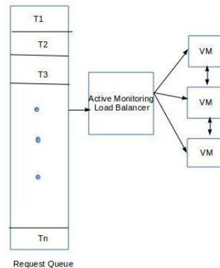
Fig.3 Active Monitoring Load Balancer
