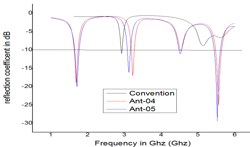
Figure 4: Reflection coefficient of conventional and DGS embedded antennas.
