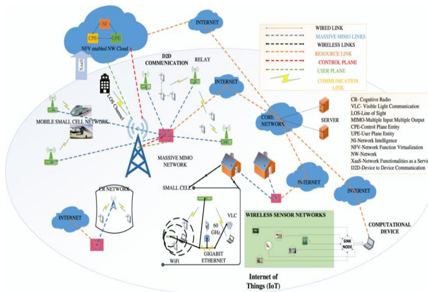
Fig. 2. 5G cellular network Architecture [1].
