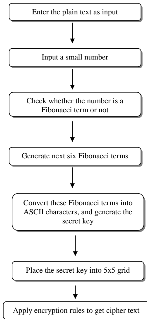
Fig. 2 Basic Steps of Proposed Algorithm
