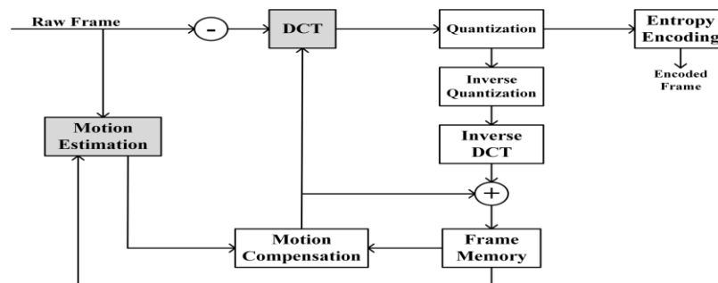
Fig. 2 Existed System
