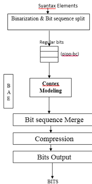
Fig. 3 Proposed System
