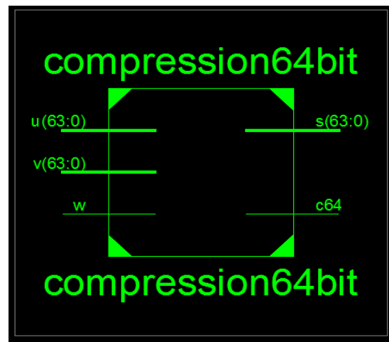
Fig.7 RTL
