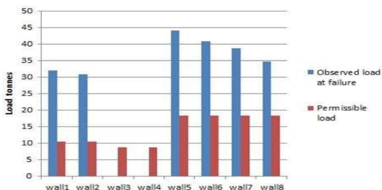
Fig.6 Compressive load at failure and permissible load for different types of walls
