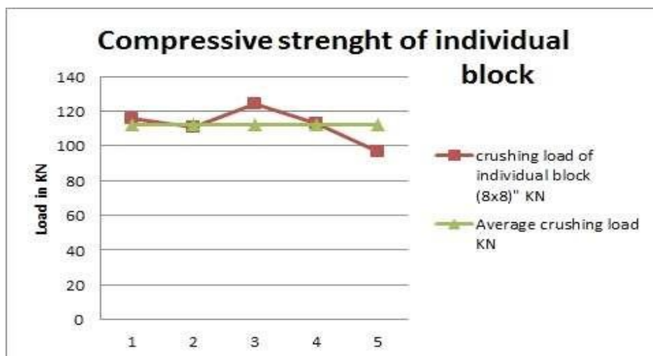
Fig.3 Compressive strength of individual hollow block of size (8x8x8) inches
