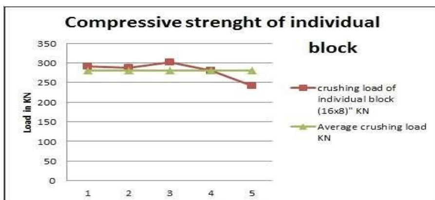
Fig.4 Compressive strength of individual hollow block of size (16x8x8) inches.
