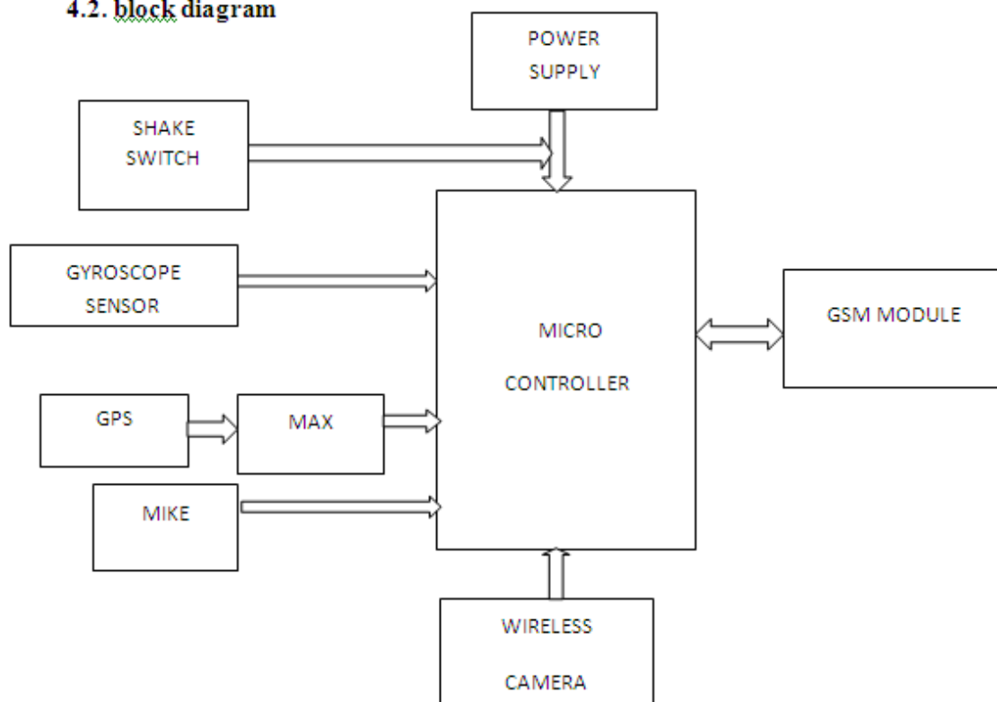
Fig 2: Block Diagram of Self Defense module
