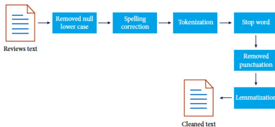
Figure 2: e- steps of the pre-processing
