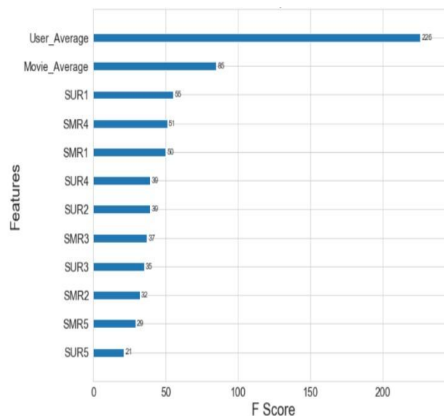
Fig.1. Feature importance of xgboost model.
