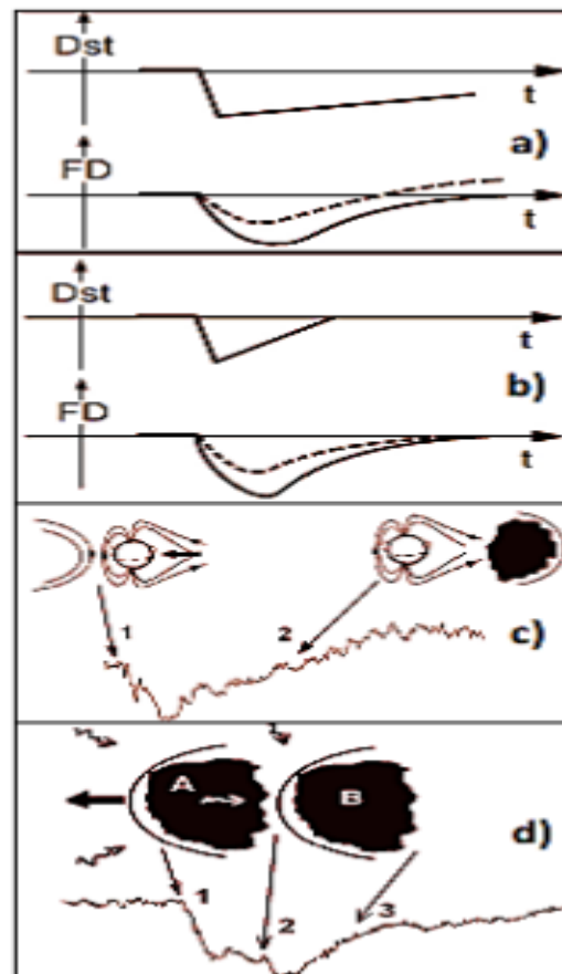
Fig. 9. Different effects of geomagnetic storm on the FD recovery: a) appearance of FD over-recovery as a consequence of Dst slow recovery (dotted line represents FD as it would look like without geomagnetic activity); b) lack of FD over-recovery due to Dst fast recovery; c) two stages of an over-recovery event, where a different CR and Dst recovery rates result in an over-recovery: commencement of FD and GMS (1) and the recovery stage (2); d) two consecutive ICMEs causing two successive depressions, the second depression showing over-recovery
