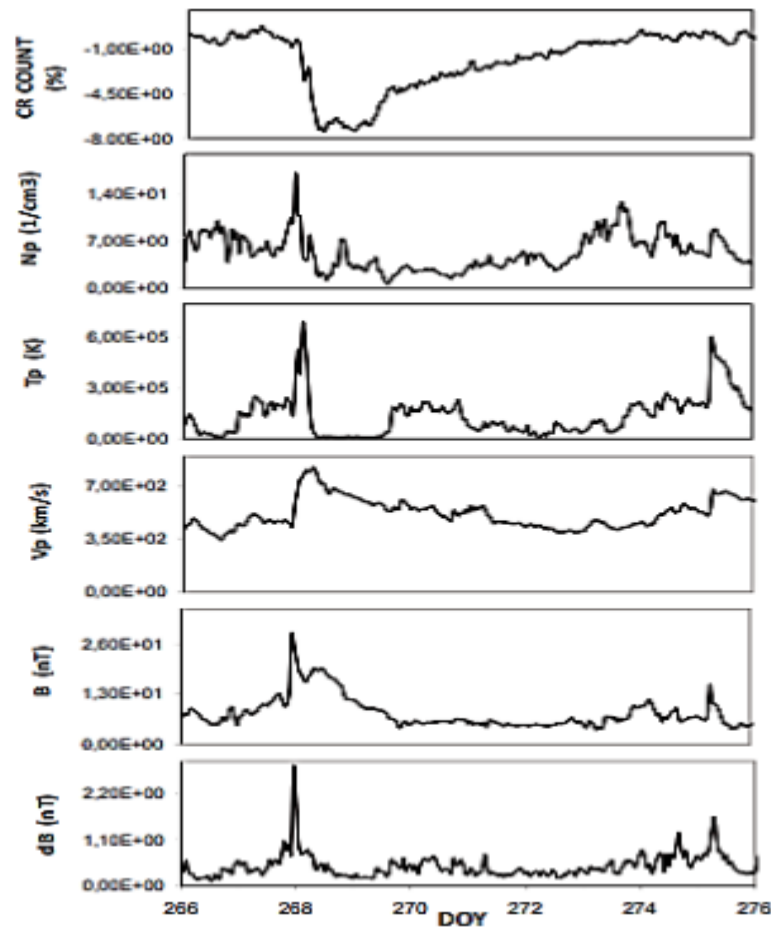
Fig. 1. ICME that arrived on 24/25 September 1998 (DOY = 268/269). The simultaneous step-increase in all the parameters is a signature of the ICME-driven shock, whereas the consecutive low-temperature region is specific for the ejection itself (e.g., Cane 2000). The CR count returns to the pre-decrease value, i.e., there is no over-recovery
