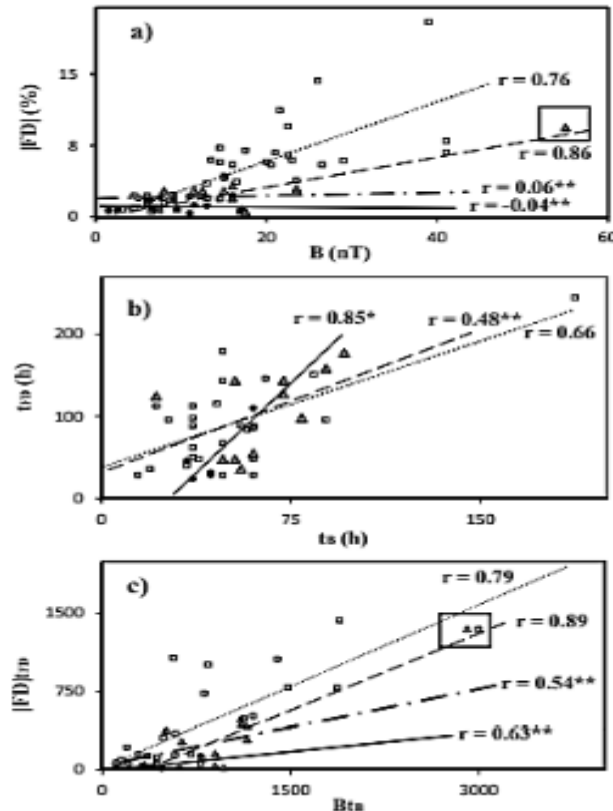
Fig. 5. Correlation of FD and SWD parameters for ICMEs (squares, dotted line), CIRs (black dots, solid line), mixed events (gray triangles, dashed line), and mixed events without outlier (circles, dashed-dotted line): a) FD
