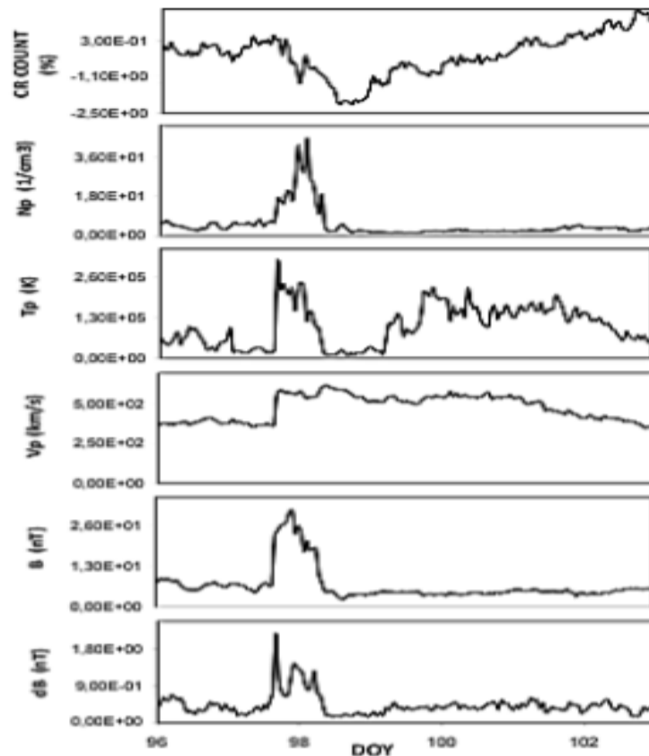
Fig. 3. ICME followed by CIR. The ICME-driven shock arrived on 06 April 2000 (DOY = 97). About two days later a new increase in speed and temperature occurred, associated with the decrease of density, which is a signature of CIR. The CR count in the recovery phase of the FD exceeds the pre-decrease level, i.e., an over-recovery is observed.
