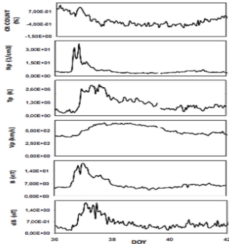
Fig. 2. CIR that occurred on 5 February 2000 (DOY = 36). The density and magnetic field peak at the forehead of the high-speed stream, whereas the increase in speed and temperature coincides with the decrease of density. The CR count in the recovery phase does not exceed the pre-decrease value, i.e., there is no over-recovery.
