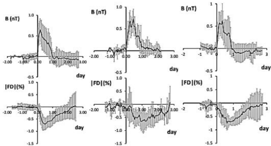
Fig. 4. Results of the superposed epoch analysis (FD magnitude, |FD| ), and magnetic field enhancement, B ) for different SWD types (left-ICMEs, middle-CIRs, right-mixed). Amplitudes in all events were normalized to 1. The time scale was normalized to the duration of the SWD magnetic field enhancement. The SEA curves are drawn with solid black lines, whereas vertical gray lines represent standard deviations over-recovery is present in a considerable number of events (see example in Fig. 3).
