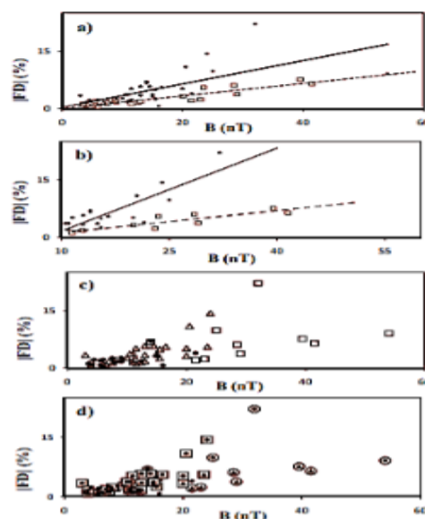
Fig. 8. Relationship between branching effect, over-recovery and geoeffectiveness as seen in |FD|(B) plot: a) over-recovery (gray squares, dotted line) and no-over-recovery events (black dots, solid line); b) the same as in
