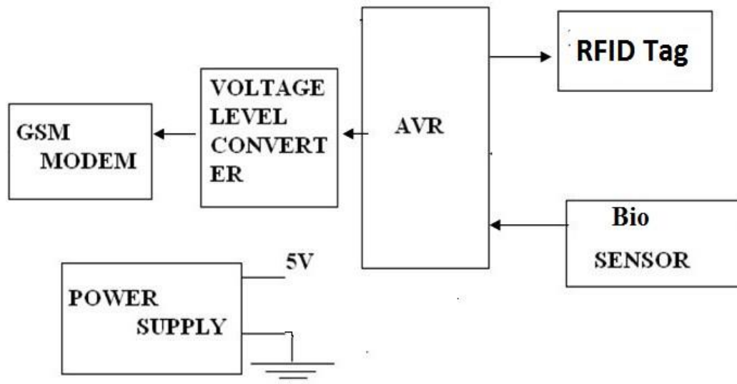
Figure 1: the block diagram of rfid based patient monitoring system.
