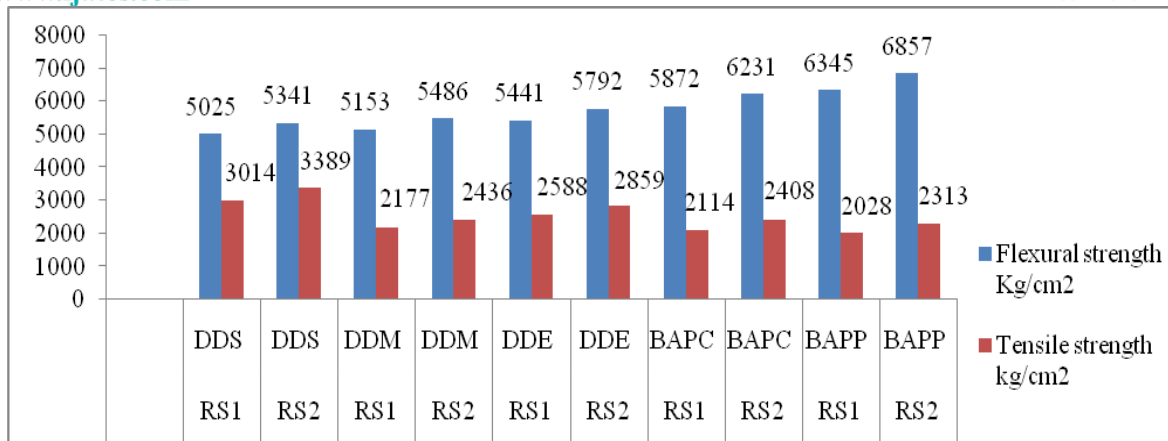
Figure 1: Comparative Data of Flexural Strength and Tensile Strength of Glass Fiber Reinforced Epoxy Blends
