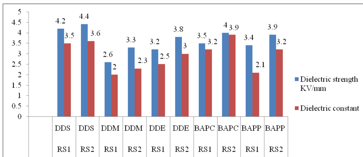
Figure 2: Comparative Data of Dielectric Strength and Dielectric Constant of Glass Fiber Reinforced Epoxy Blends
