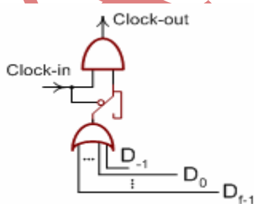
Fig 4: The multiple bit clock gator logic.
