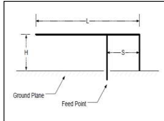
Figure 2: Inverted-F Antenna Geometry.
