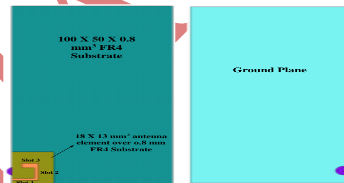
Figure 7: Top and Bottom View.
