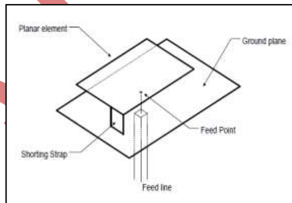
Figure 4: Basic layout of the planar inverted-F antenna.
