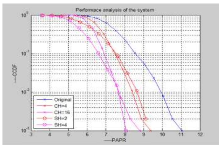
figure 4: the papr reduction performance of switching hybrid scheme for ofdm systems.
