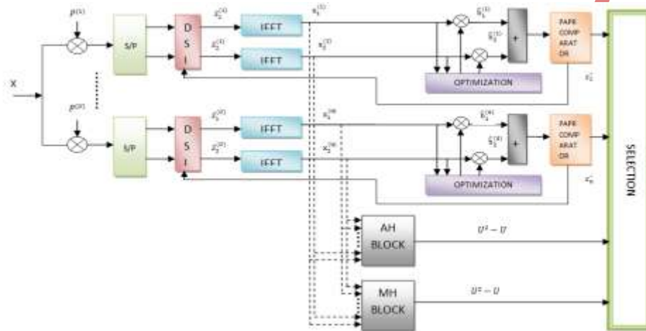
figure 1: block diagram of dummy signal hybrid scheme
