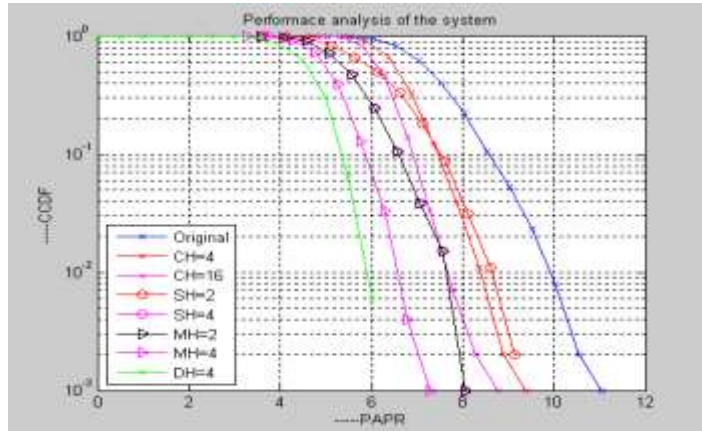
figure 6: the papr reduction performance of dummy signal hybrid scheme for ofdm systems.
