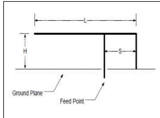
Figure 2: Inverted-F Antenna Geometry.
