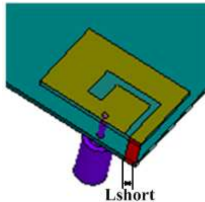
Figure 8: Suspended View.
