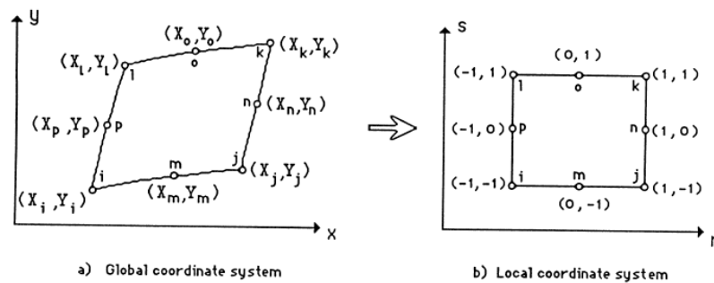
Fig 4.1 Co-ordinate system
