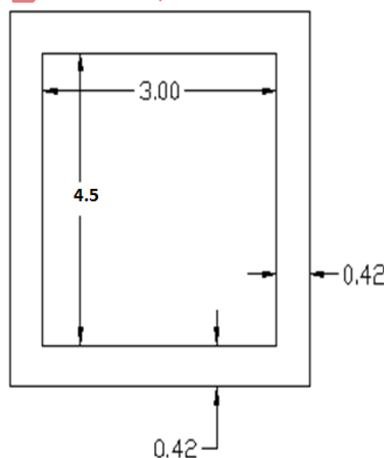
Fig 5.1 Box Culvert (All dimension in meter)
