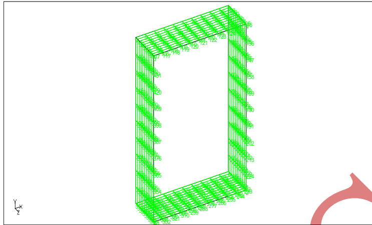
Fig 5.2 STAAD Model of Box Culvert
