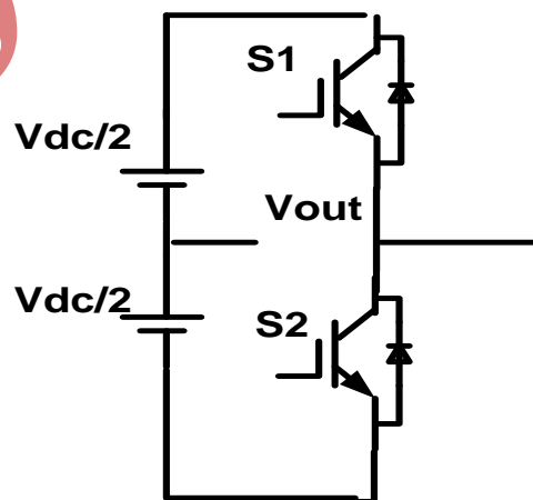
Figure 7 Half Bridge
