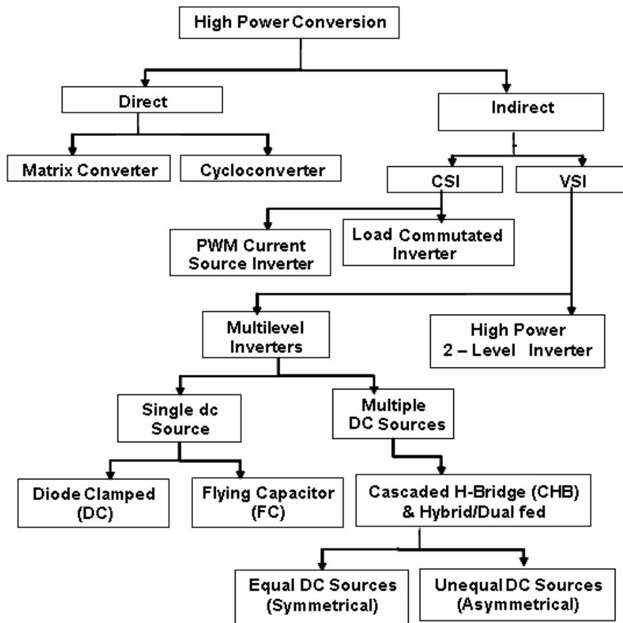
Figure 6 Classifications of High Power Converters
