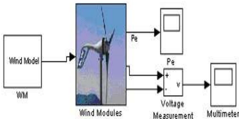
Fig 3 : Equivalent Circuit for Modeling of Wind System
