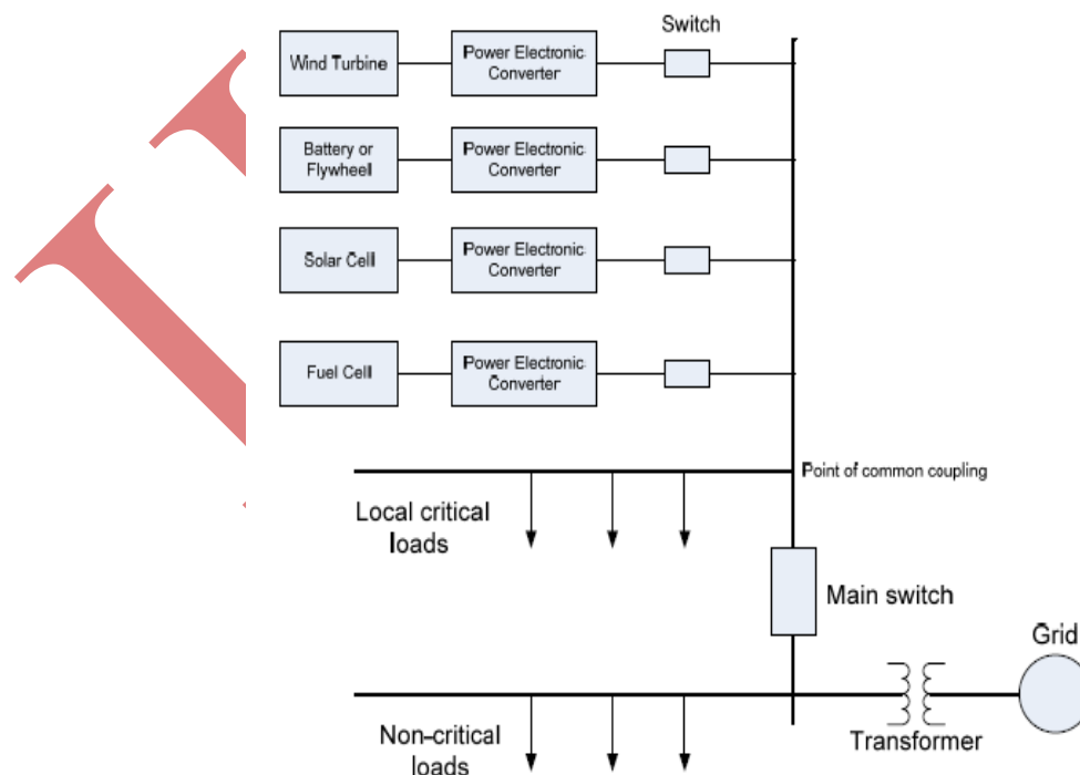
Fig. 1 A Schematic Diagram of a Micro Grid
