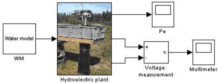
Fig 4 : Equivalent Circuit for Modeling of Hydro System
