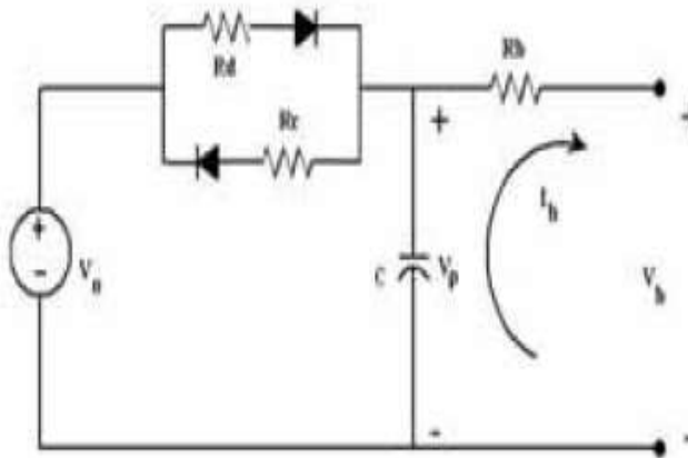
Fig 5 : Equivalent Circuit for Modeling of Battery
