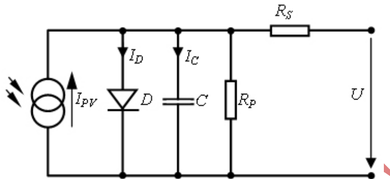
Fig 2 : Equivalent Circuit for Modeling of PV System
