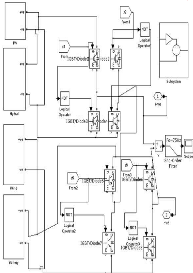
Fig 9: Matlab/Simulink Model of Micro Grid
