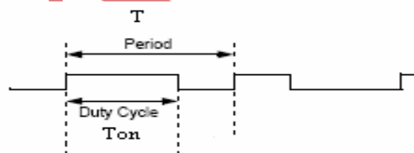
Fig.2 PWM Signal
