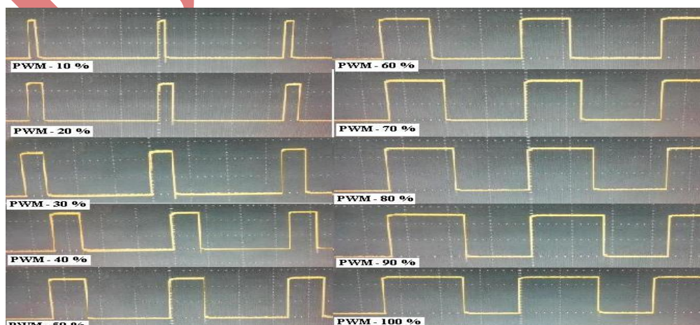
Fig.3 PWM Waveform At 10 To 100 % on DSO
