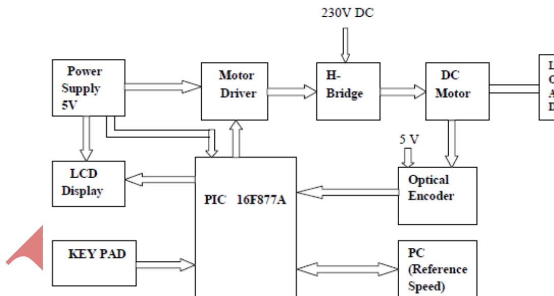
Fig.9 Functional Block Diagram
