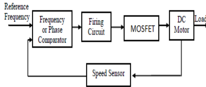
Fig.1 Block Diagram of DC Motor Speed Control by Using MOSFET
