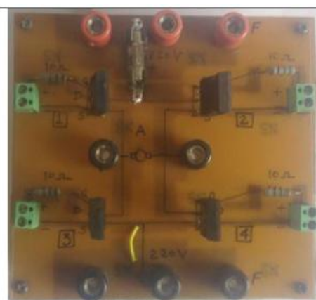
Fig.8 Actual H-Bridge Circuit
