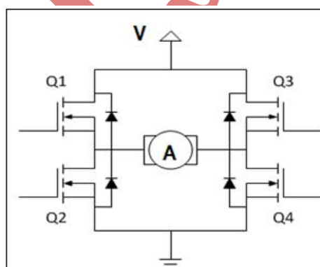
Fig.7 H-Bridge
