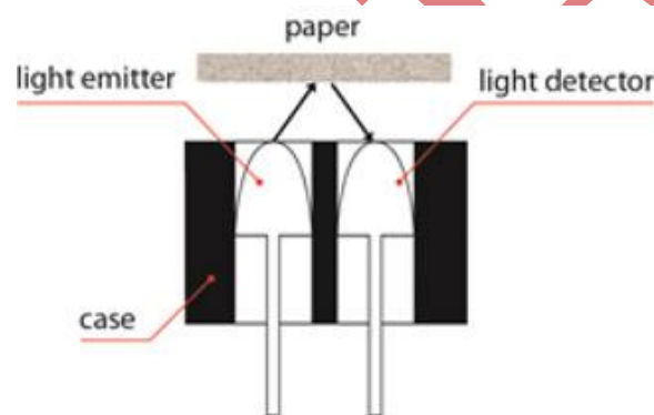
Fig.5 Optical Encoder
