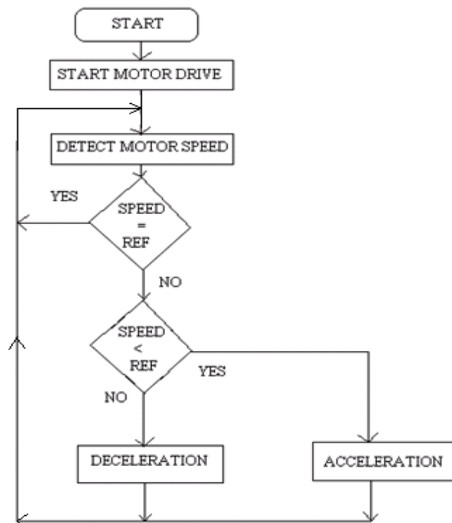
Fig.10 Basic Flow Chart of DC Motor Speed Control
