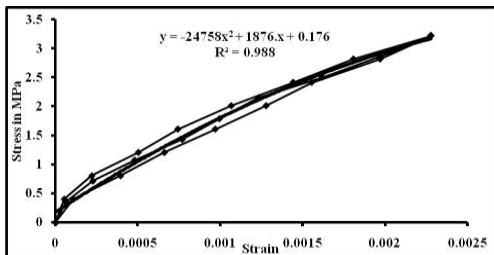
Fig. 9 Modulus of elasticity at 28 days of series H9[50:40:10][Sand]
