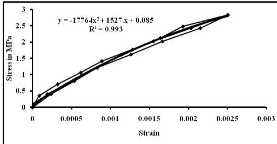
Fig. 10 Modulus of elasticity at 28 days of series H11[55:35:10][Sand]
