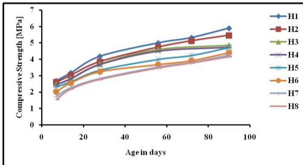
Fig. 1 Variation of Compressive Strength with age with quarry dust as fine aggregate
