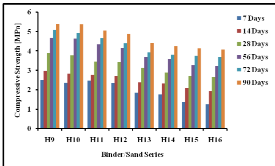
Fig. 4 Compressive Strength of H9 to H16 of Binder/Sand Series for various ages
