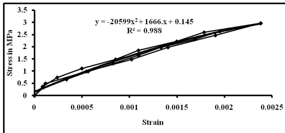
Fig. 7 Modulus of elasticity at 28 days of series H1[50:40:10][QD]
