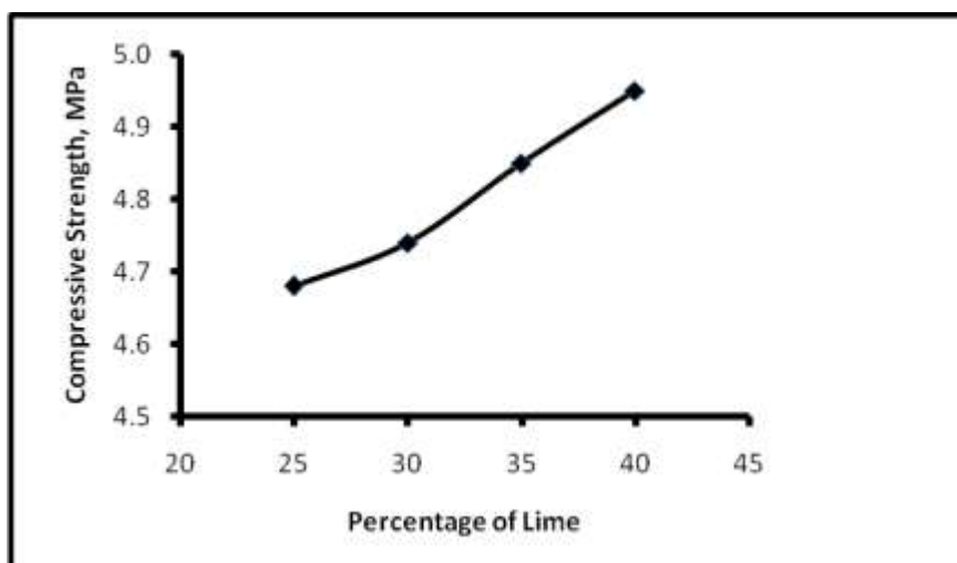
Fig. 6 Variation of Compressive Strength with lime content
