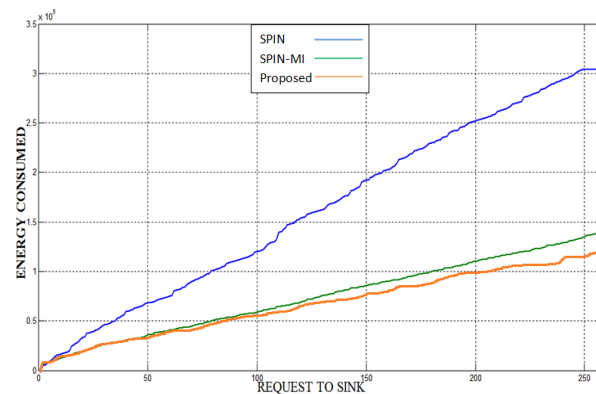
Fig2. Overall Energy Consumption of Sensor Network
