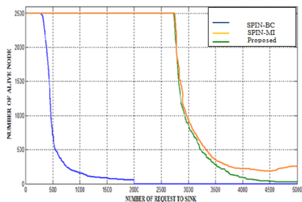
Fig1. Number of Alive Node in the Sensor Network
