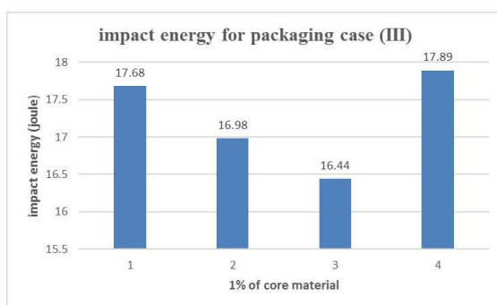
Fig.6 impact energy for 1% of core material
