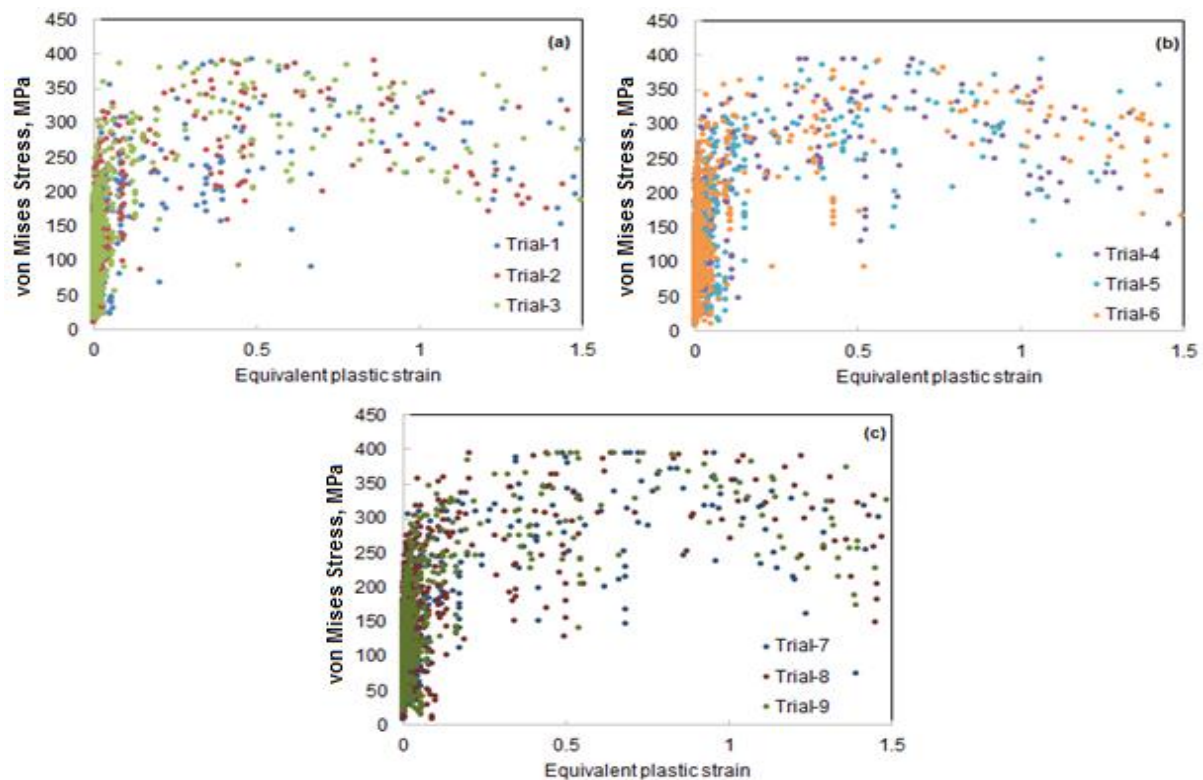
Figure 3: Effect of equivalent plastic strain of von Mises stress
