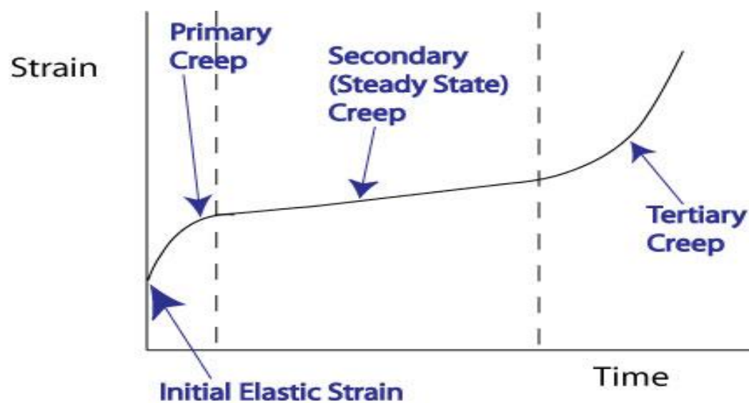
Figure1: (Stages Of Creep)
