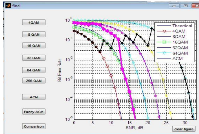
Figure 4.3: Comparison of Fuzzy ACM and Conditions Based ACM
