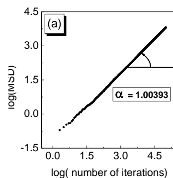
Figure 4. Plot of MSD vs t for Compact Clusters plotted on log-log scale.
