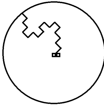
Figure 1. Basic Random Walk for Aggregation in DLA
