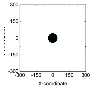
Figure 2. Compact Cluster of N = 5000
