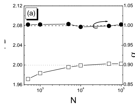
Figure 5. Plot shows the variation of FD and \alpha against N particle number for a compact cluster. From Fig. 5 it is clear that the value of exponent \alpha depends on cluster dimension (FD) and not on the size ( N ) of the cluster.
