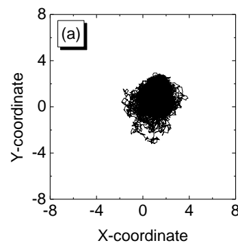
Figure 3. Motion of CM of Compact Cluster
