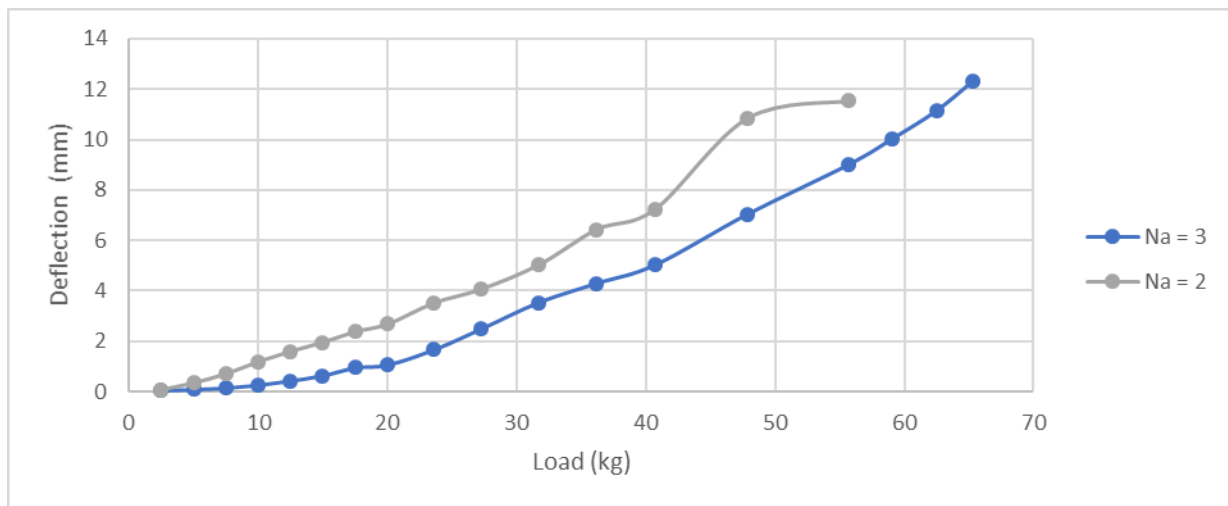
Fig. 2. Effect of number Anchors ( N_a )
