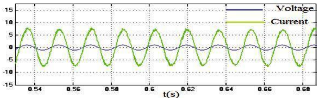
Fig.7 Voltage and Current are in Phase Using PI Controller
