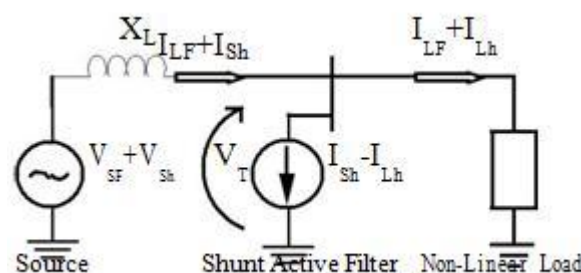
Fig.1 Principle of Shunt Current Compensation
