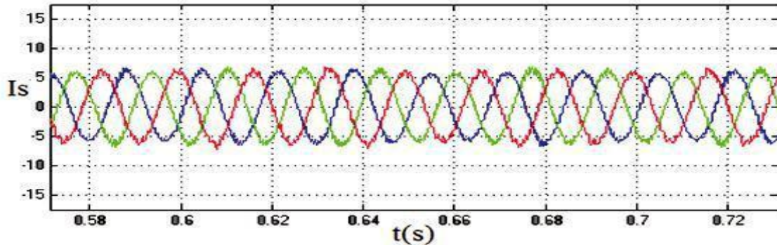
Fig.5 Compensating Current of PI Controller.
