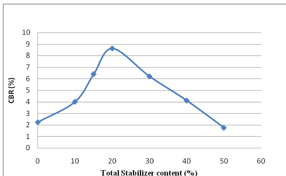
GRAPH-2 Change in CBR (%) with increase in total stabilizer (%)
