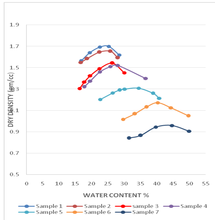
GRAPH-1 Moisture density relationship for different samples
