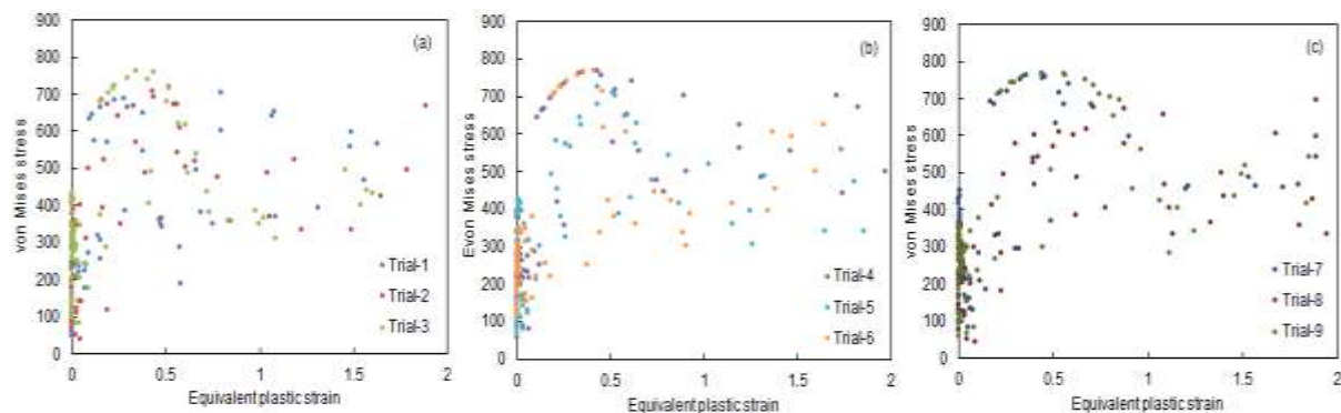
Figure 4: Effect of equivalent plastic strain on von Mises stress: (a) 1.0 mm, (b) 1.2 mm and (c) 1.5 mm sheet thickness.
