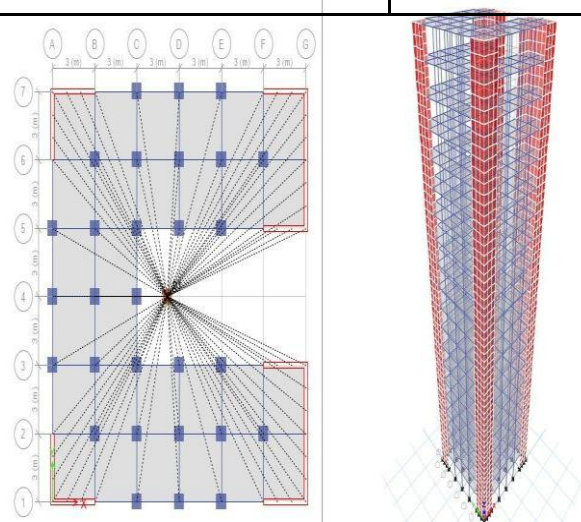
Fig. 2. Plan of shear wall system C-Section building
