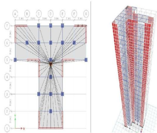
Fig. 2. Plan of shear wall system T-Section building
