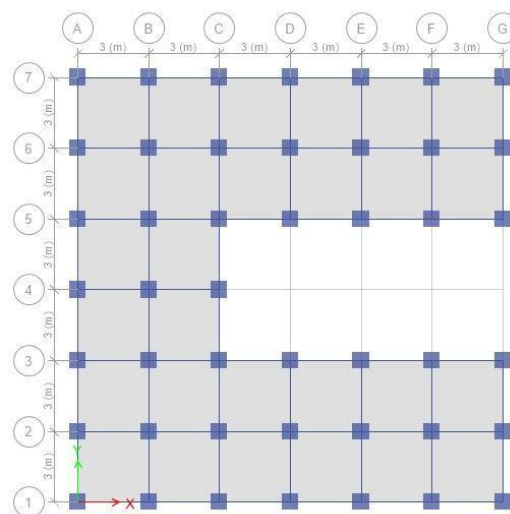
Fig. 1. Plan of Moment Resisting Frame C-Section building
