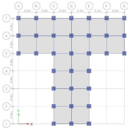
Fig. 1. Plan of Moment Resisting Frame T-Section building
