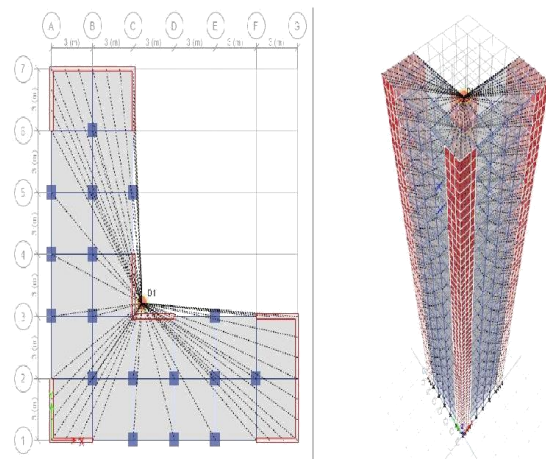
Fig. 2. Plan of shear wall system L-Section building
