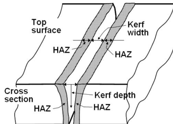
Fig. 2.1 Principle of Laser cutting
