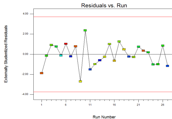
Fig. 5.2 Residual Vs Run graph
