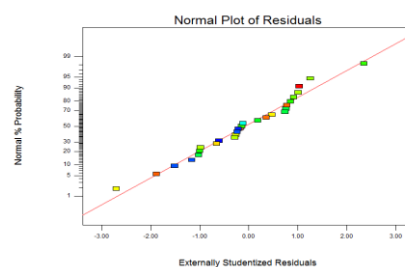
Fig. 5.1 Normal probability plot of residuals for Kerf Width
