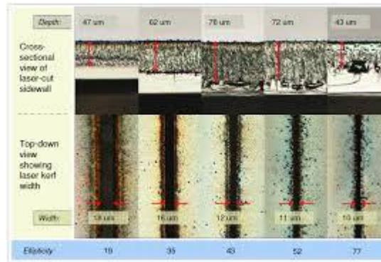
Fig. 4.2 Response of Kerf width
