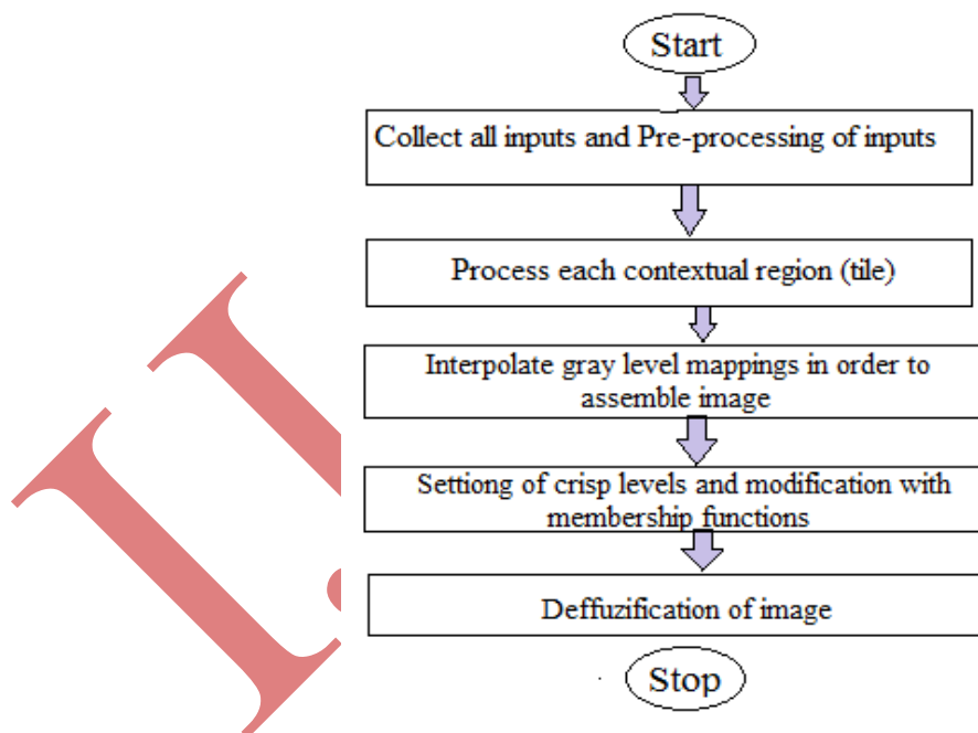
Fig 2 Flow Chart of CEFHE
