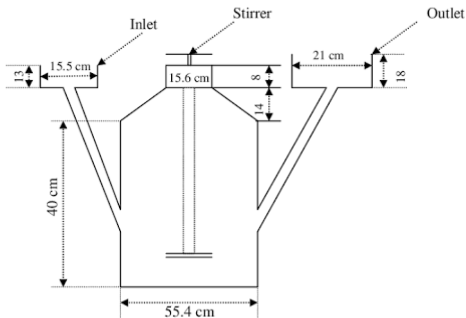
Fig.1: Schematic diagram of bio-digester
