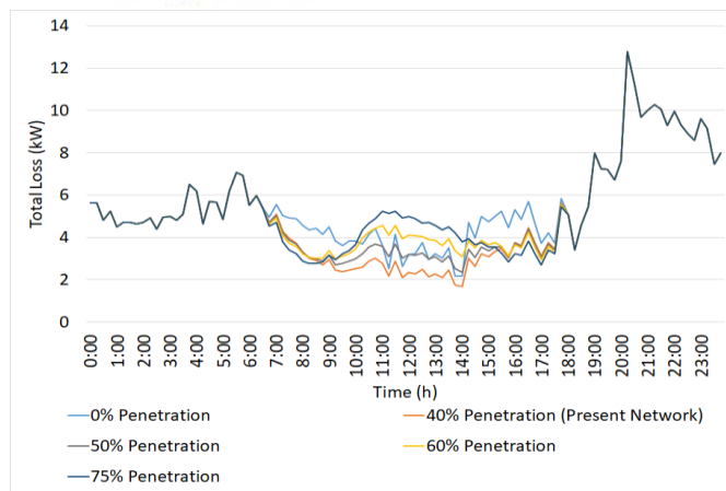
Fig. 7. Network Power Losses.
