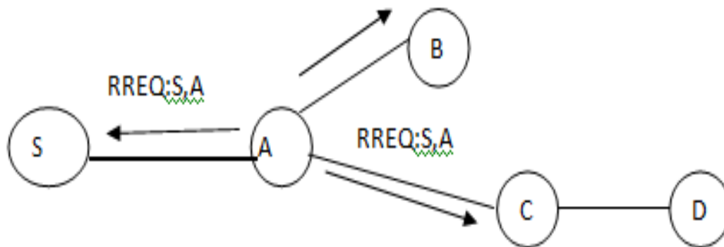
Fig3:ROUTEREQUEST(SneedsaroutetoD)
