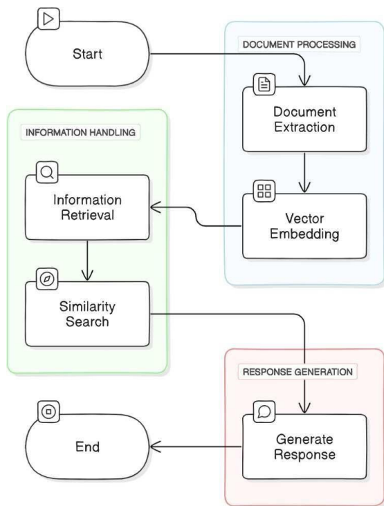
Fig. 3. Chatbot Implementation
